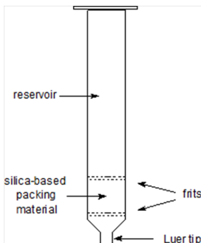
Fig. 5: Representation of SPE Tube.
